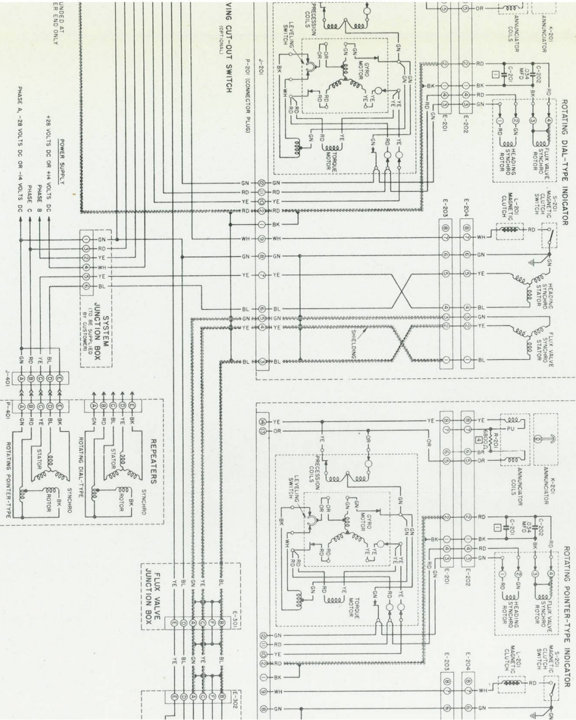
FIGURE 5-1 GYROSYN SCHEMATIC WIRING
